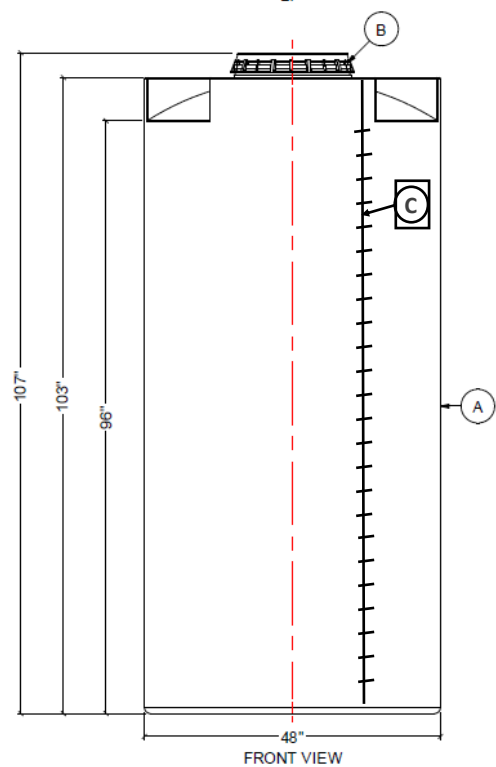
FRONT VIEW
